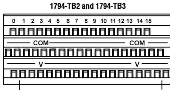
V = 24V dc COM = 24V dc common These terminals on 1794-TB3 only.
