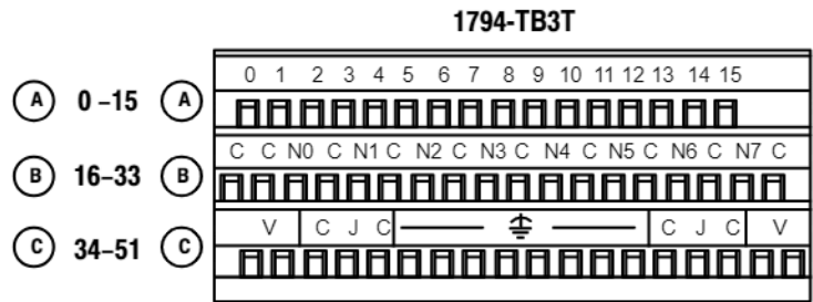
Where: V = 24V dc C = 24V dc common CJC = cold junction compensation N = additional input ⏏ = chassis ground
